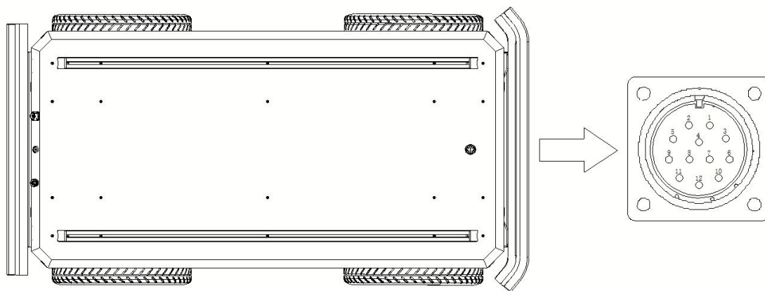
Figure 3-4 Top Electrical Interface Layout Diagram
